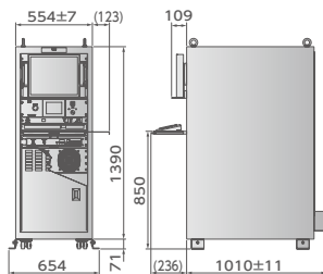
● CRD-2000W
