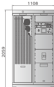
● CRD-2000W
