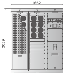
● CRD-2000T
